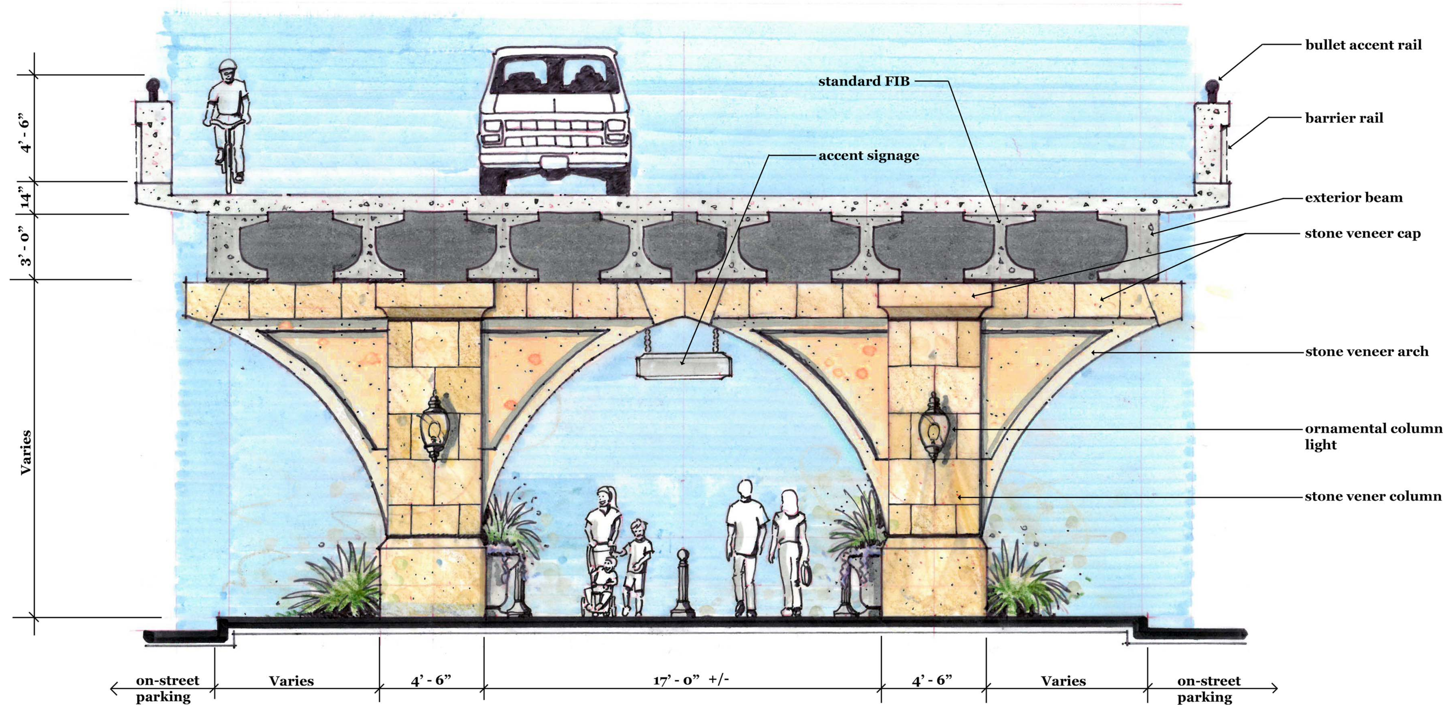
B Bridge Pier Column - Elevation N.T.S. *Finishes & features to be determined based on established budget developed for project
