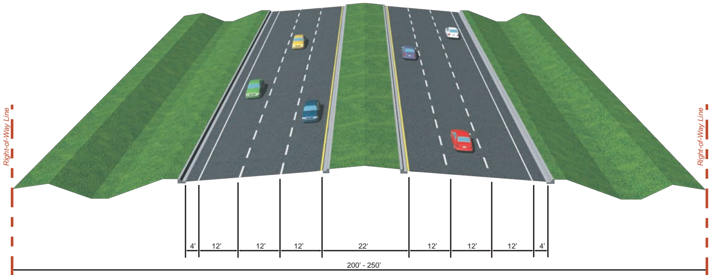
6 - LANE URBAN TYPICAL SECTION From SR 207 to CR 214
