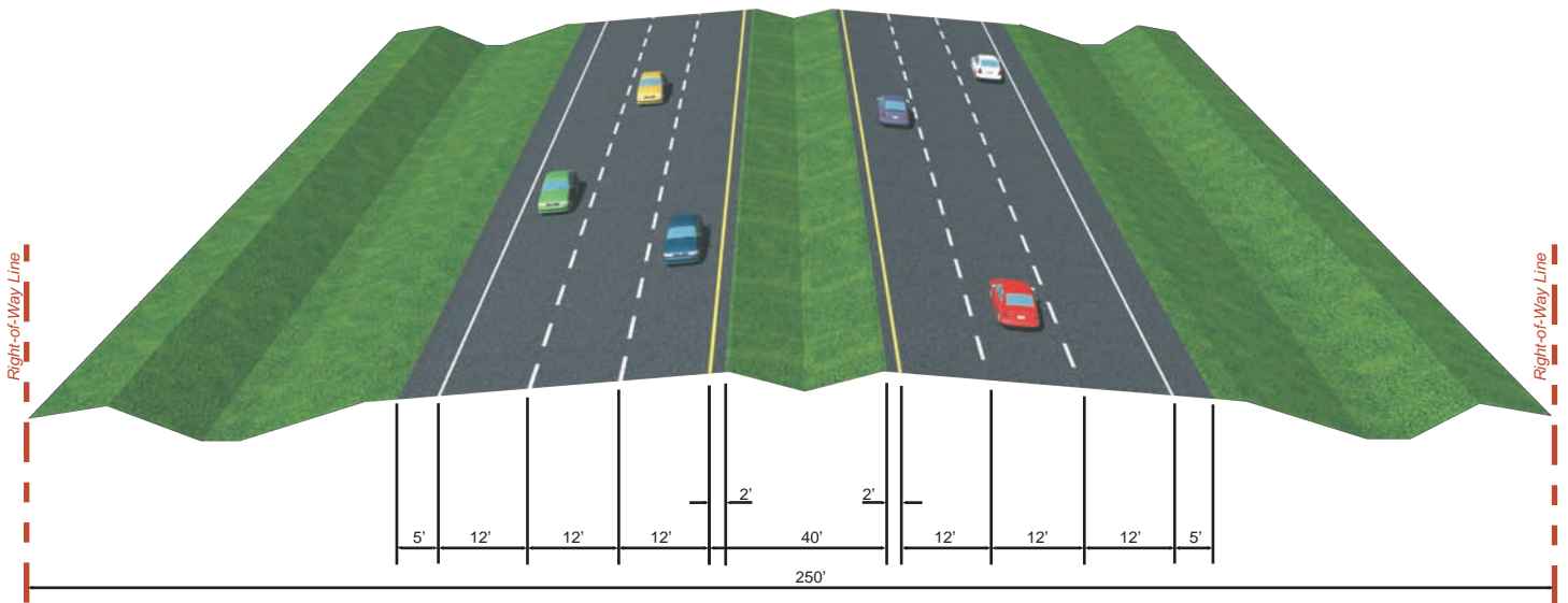
6 - LANE RURAL TYPICAL SECTION From CR 214 to SR 16
