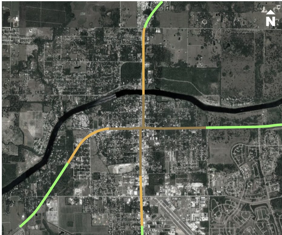
FIGURE 10 DISTINGUISHING CONTEXT CLASSIFICATION SEGMENTS BY DEVELOPMENT INTENSITY AND ROADWAY NETWORK
