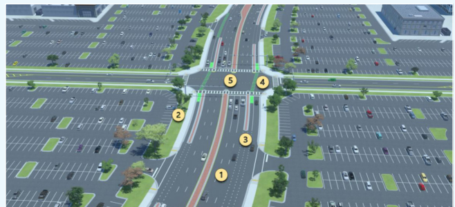
FIGURE 21 C3C-SUBURBAN COMMERCIAL SPEED MANAGEMENT
