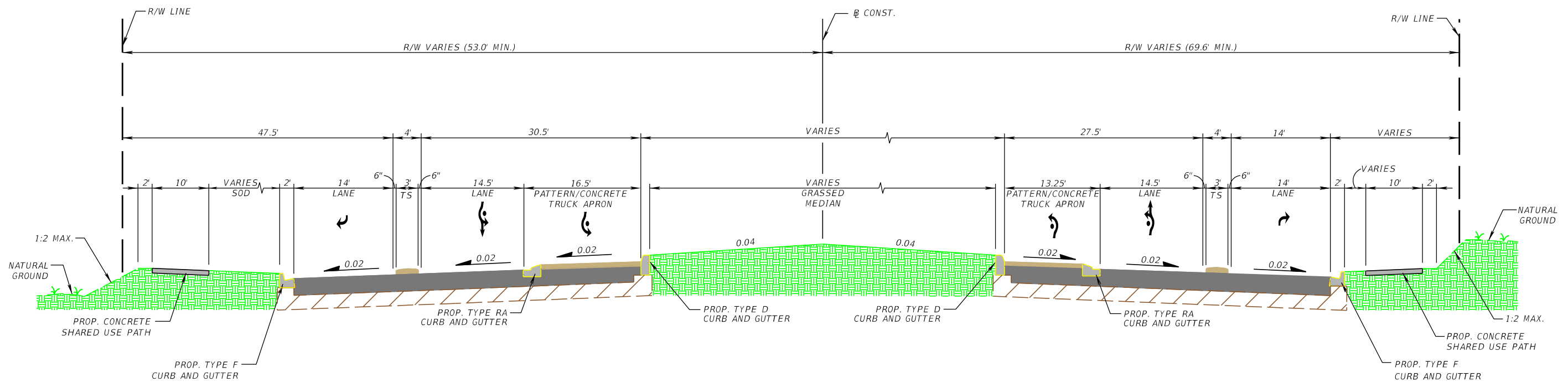
TYPICAL SECTION No. 2 SR 109 (UNIVERSITY BLVD.) AT MERRILL ROAD STA. 104+38.00 TO STA. 105+77.31
