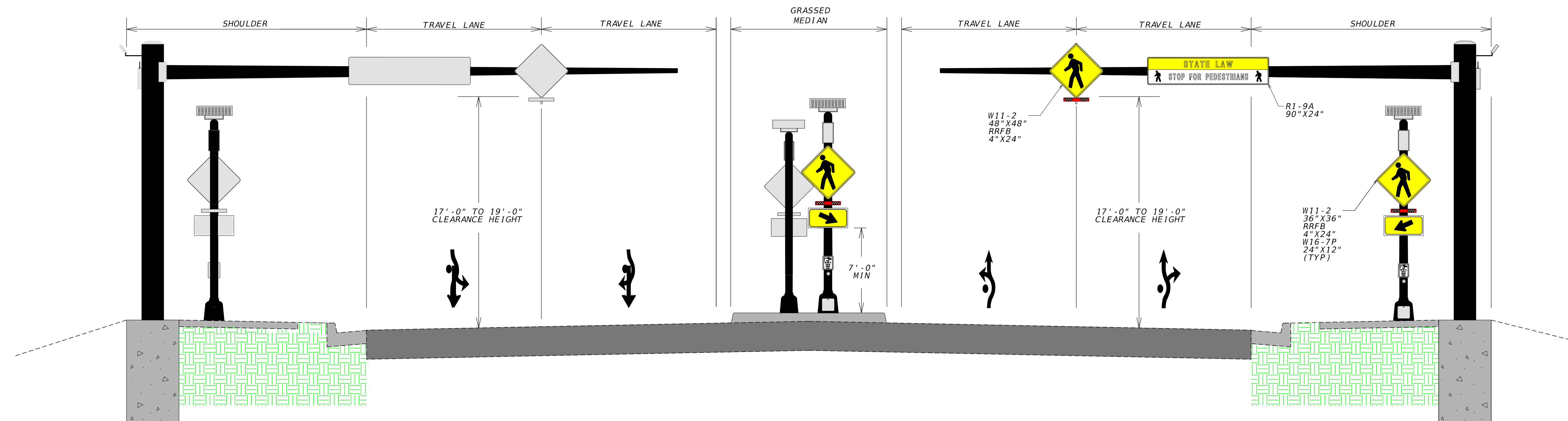
TYPICAL SECTION OF RRFB INSTALLATION SR 109 (UNIVERSITY BLVD) AT MERRILL ROAD ROUNDABOUT
