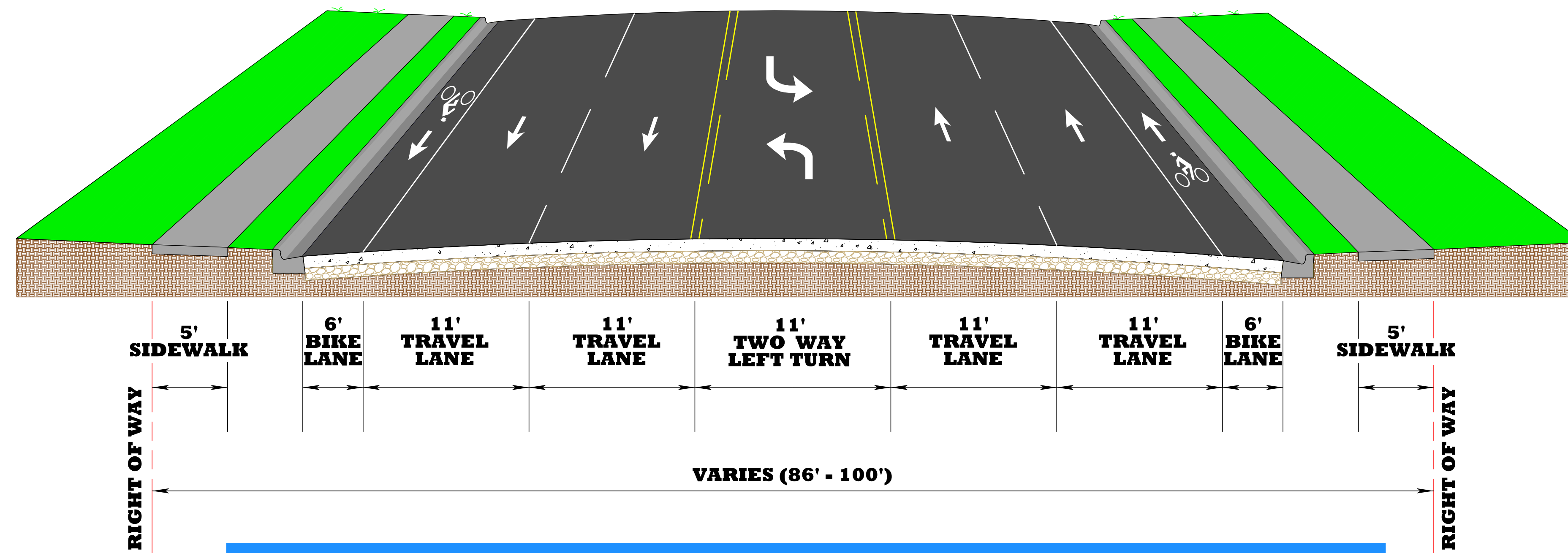
PROPOSED ROADWAY TYPICAL SECTION
