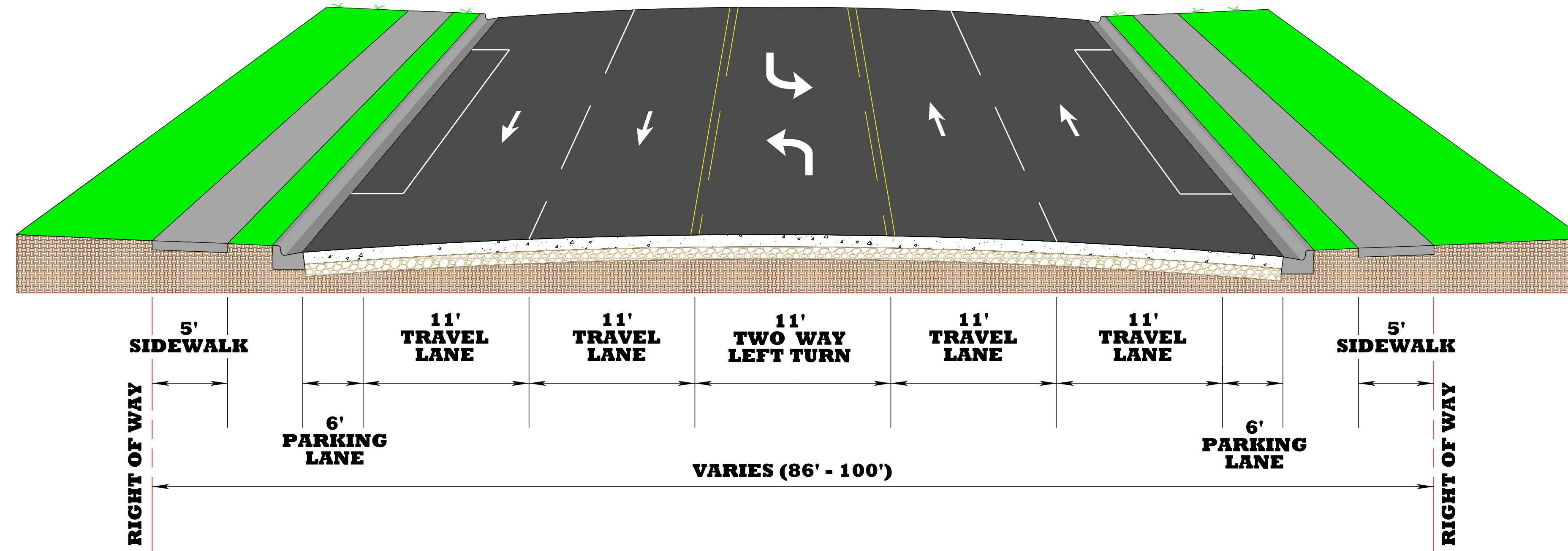
EXISTING ROADWAY TYPICAL SECTION
