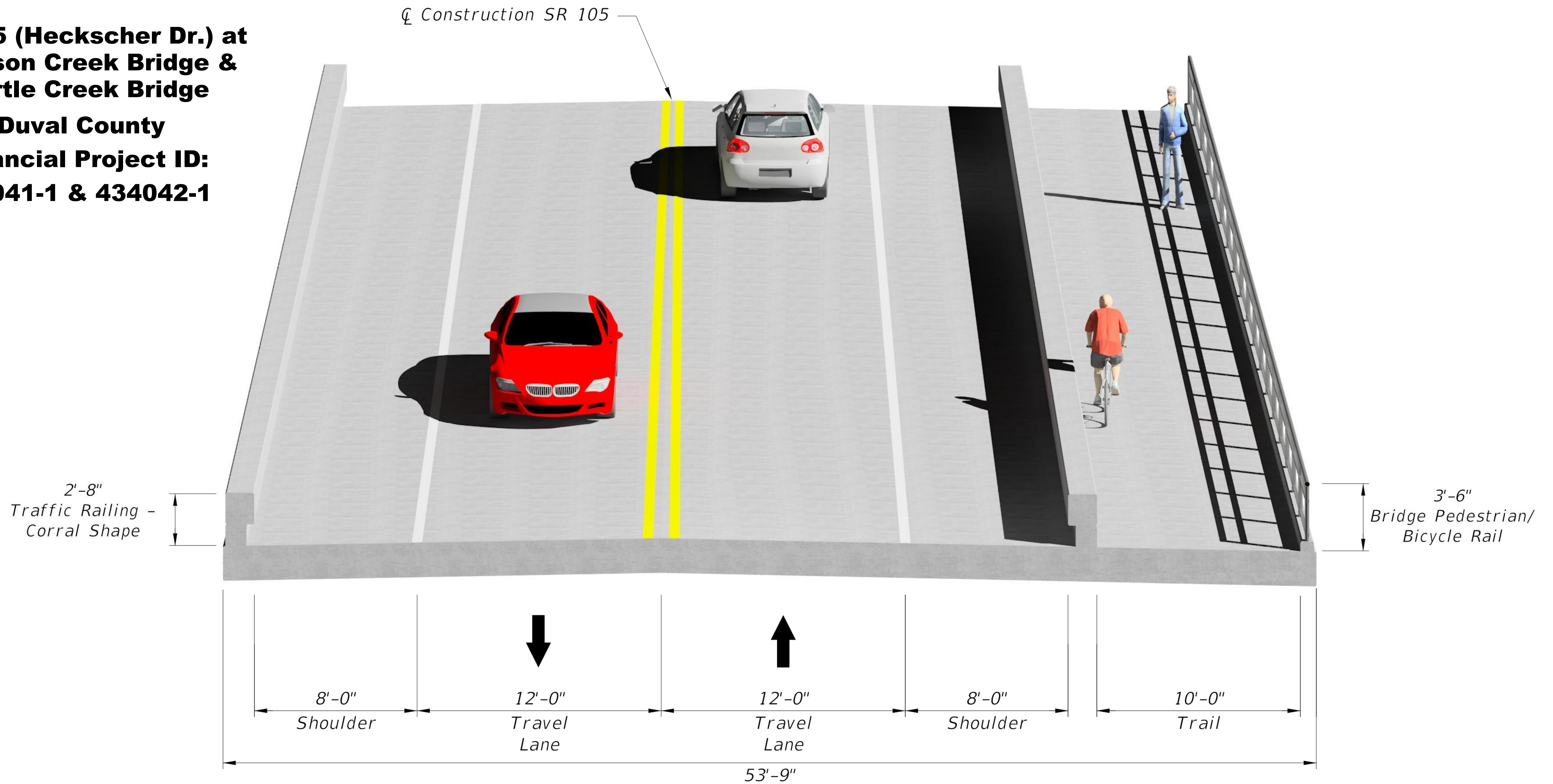
BRIDGE TYPICAL SECTION
