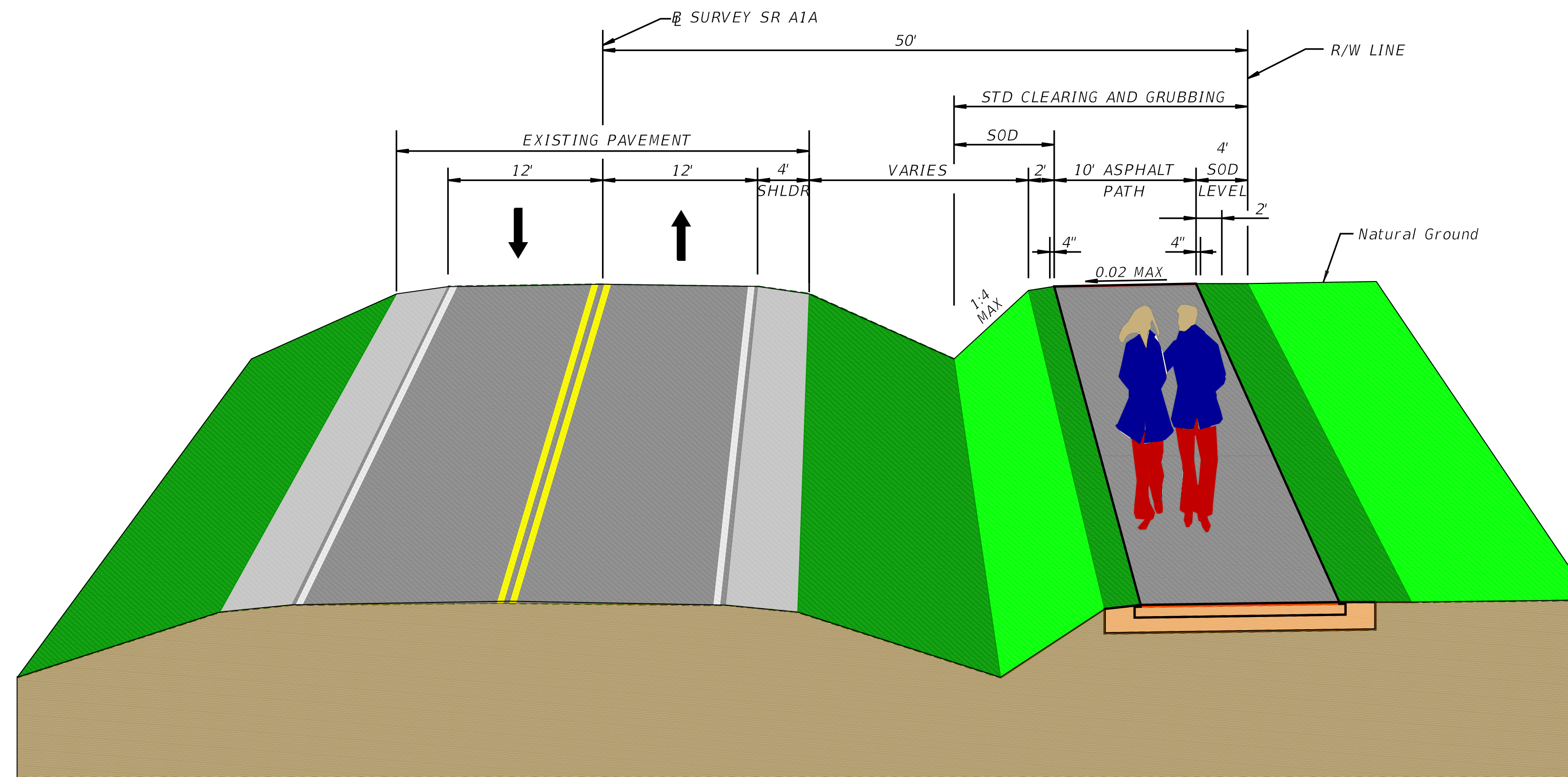
TYPICAL SECTION NO. 2 FROM 480' SOUTH OF FORT GEORGE ROAD TO FORT GEORGE ROAD
