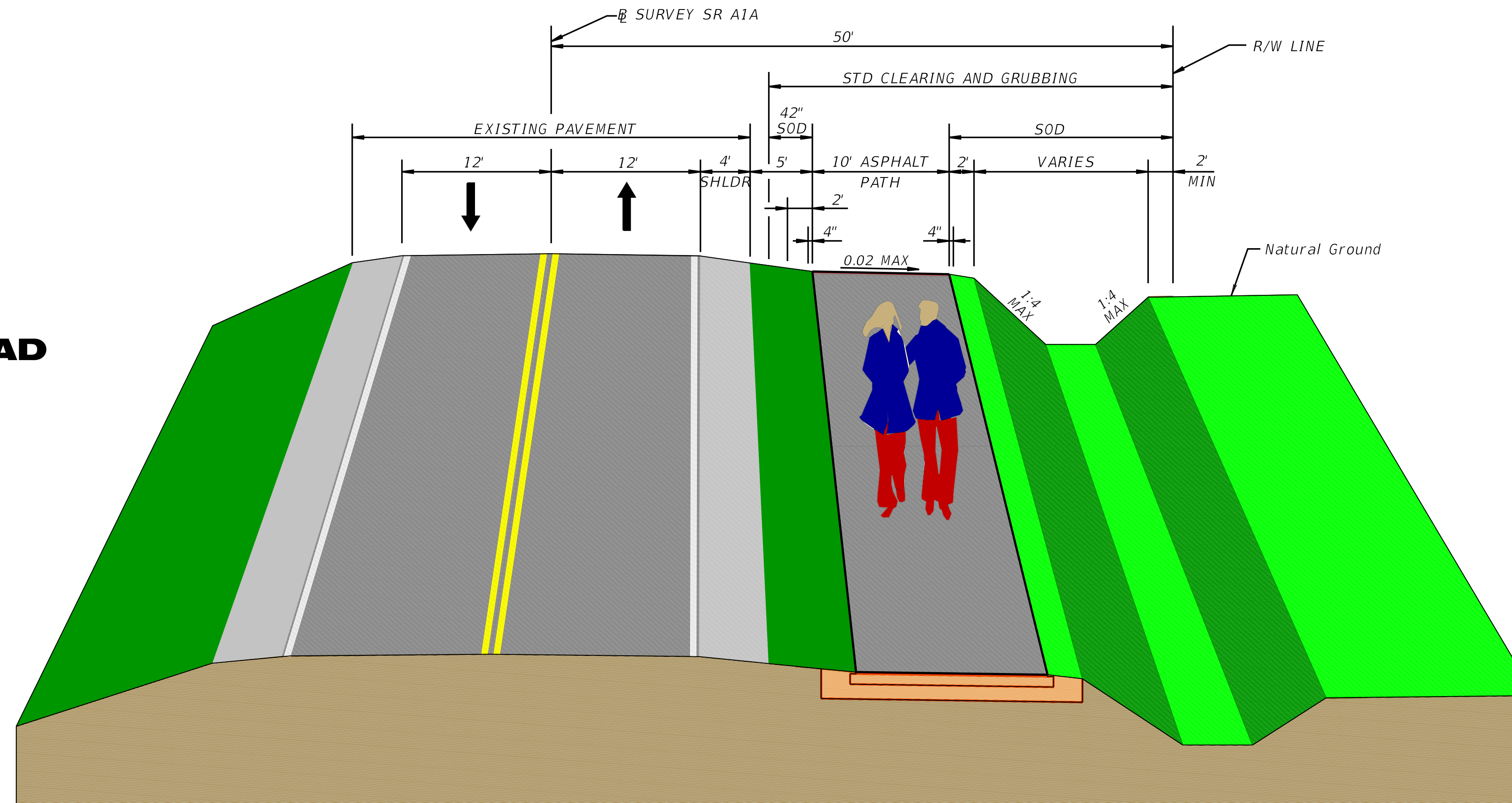
TYPICAL SECTION NO. 1 FROM SANDOLLAR RESTAURANT TO 480' SOUTH OF FORT GEORGE ROAD FROM FORT GEORGE ROAD TO CHAPMAN'S PLACE
