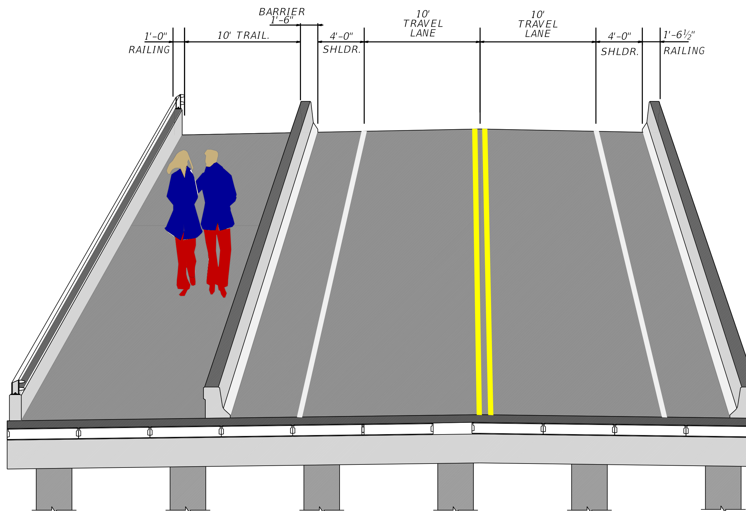
BRIDGE TYPICAL SECTION OPTION 2
