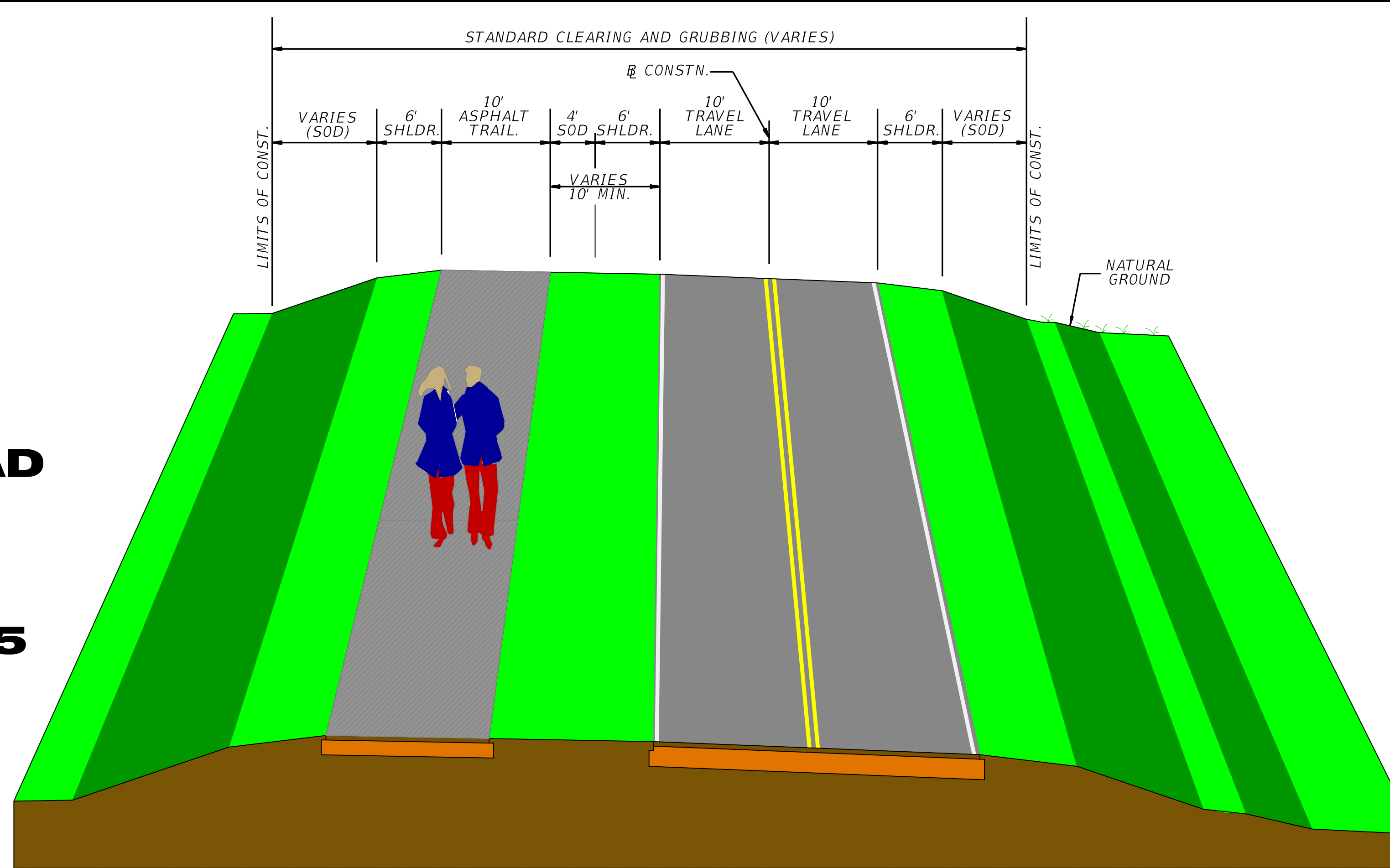
ROADWAY TYPICAL SECTION OPTION 1
