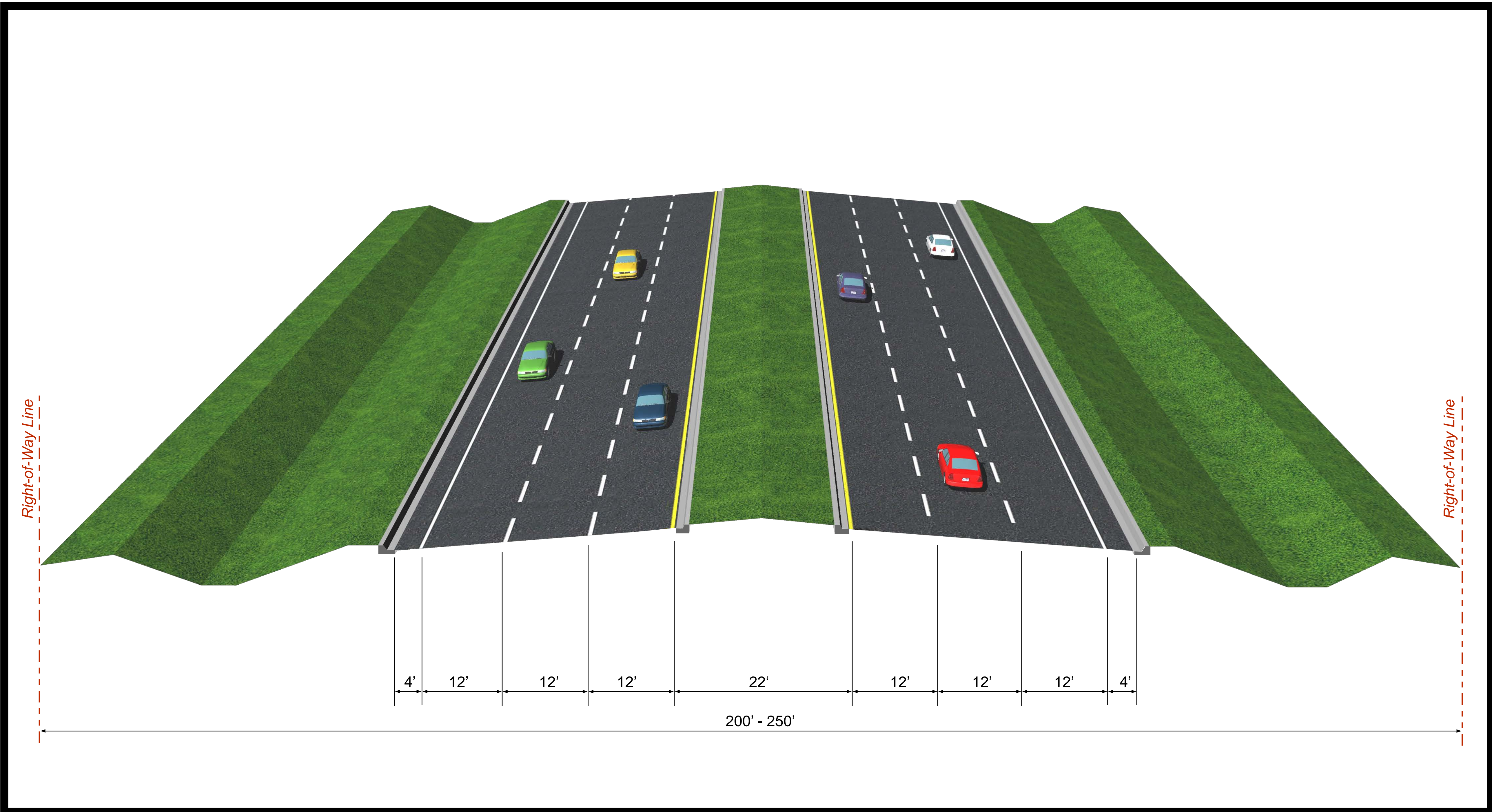
SR 313 6 - LANE URBAN TYPICAL SECTION South of SR 207 to CR 214
