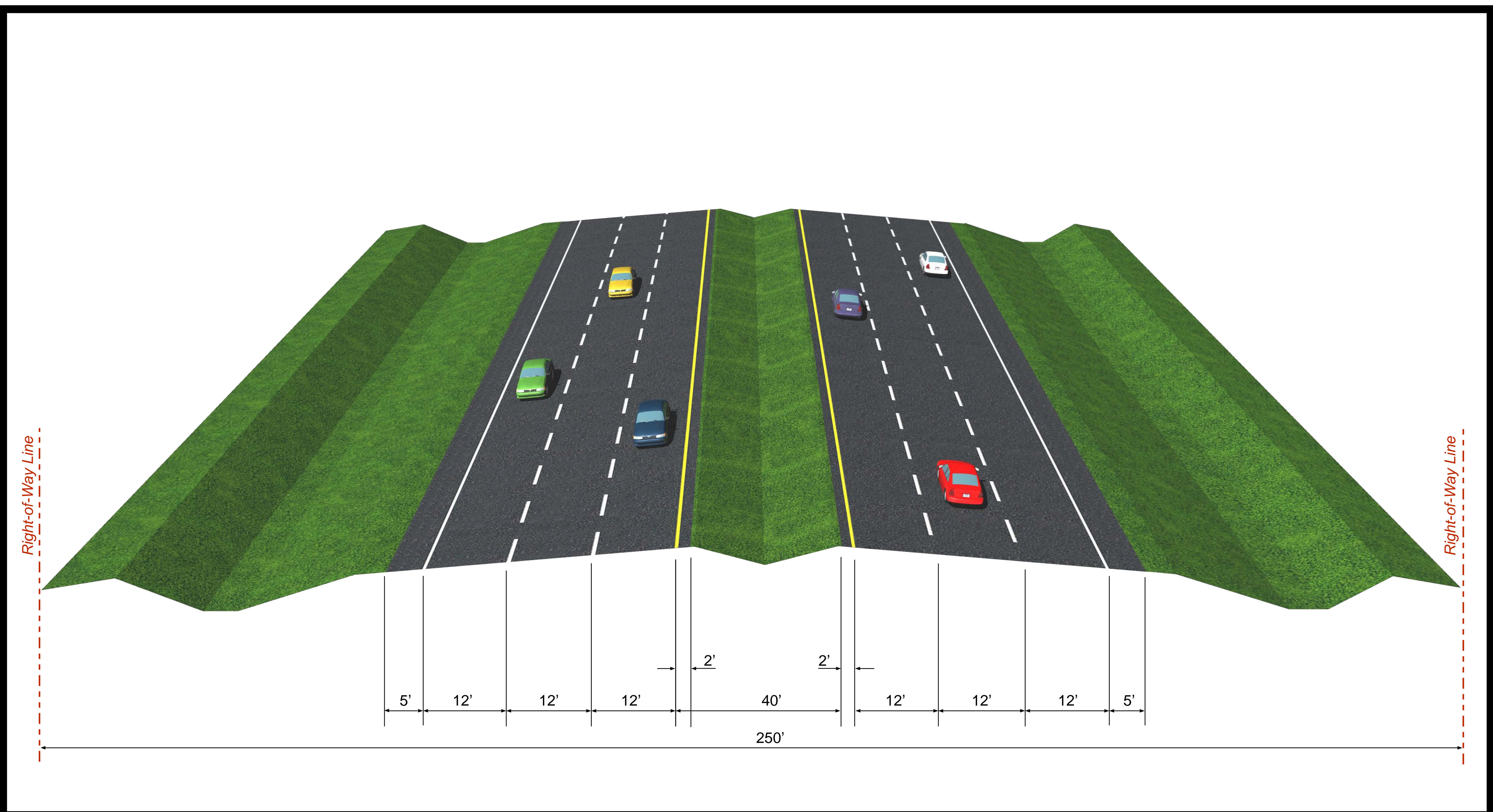
SR 313 6 - LANE RURAL TYPICAL SECTION From CR 214 to SR 16
